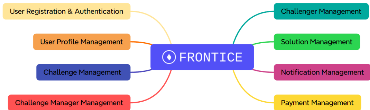
Figure 3 - 2 Functional Requirements
