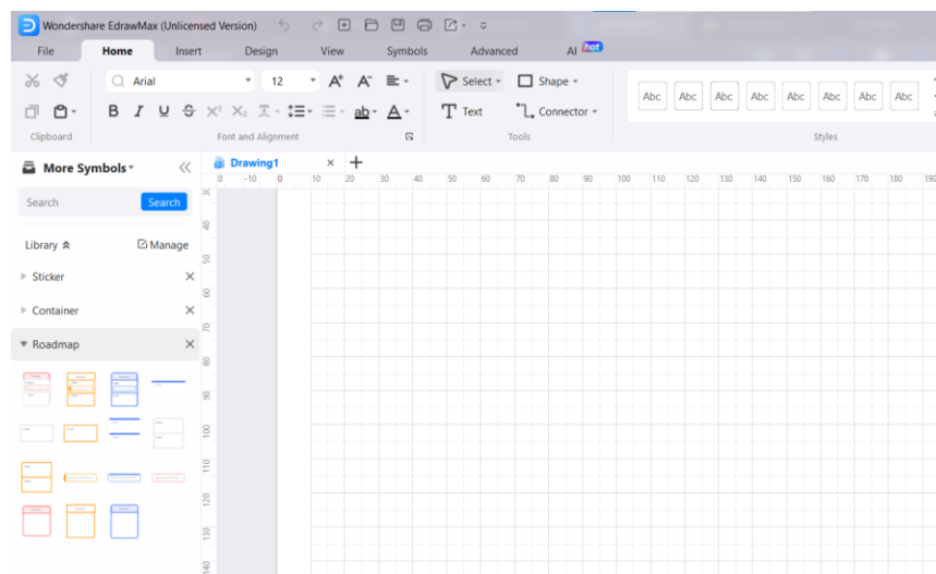
Figure 2 - 12 EdrawMax
