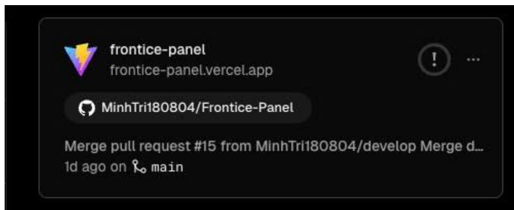
Figure 7 - 4 Deploy Vercel
