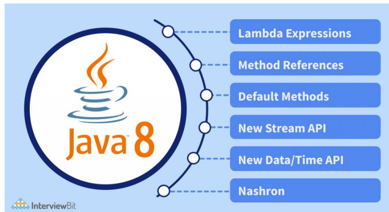
Figure 2 - 1 Java 8 (InterviewBit)
