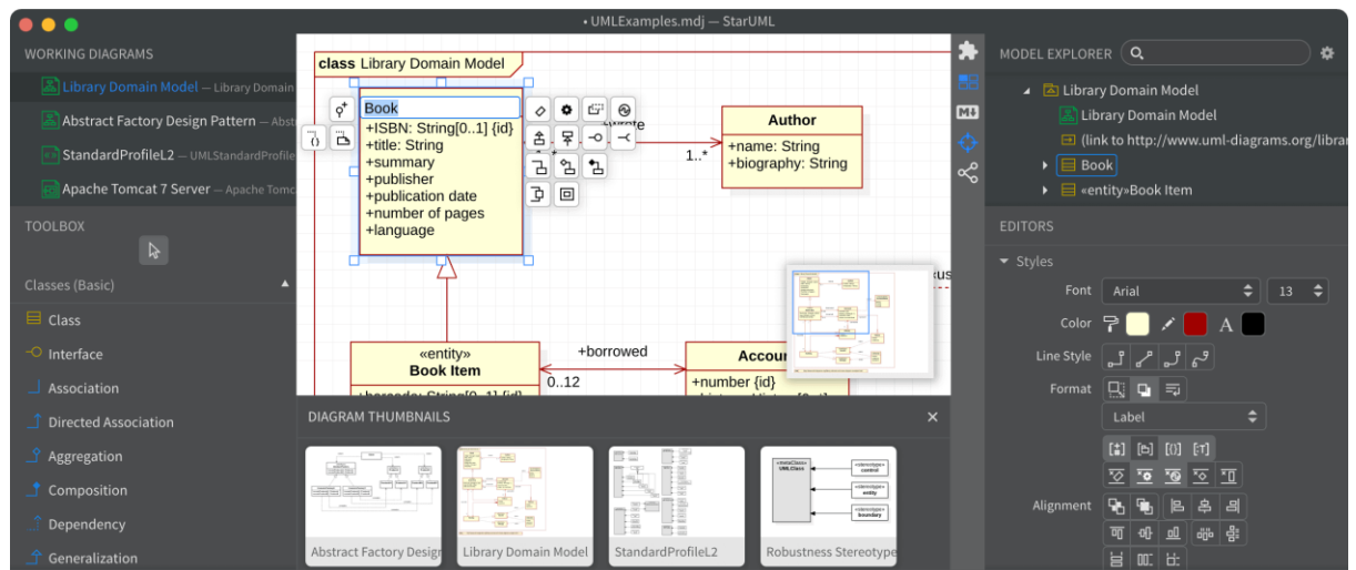
Figure 2 - 11 Start UML
