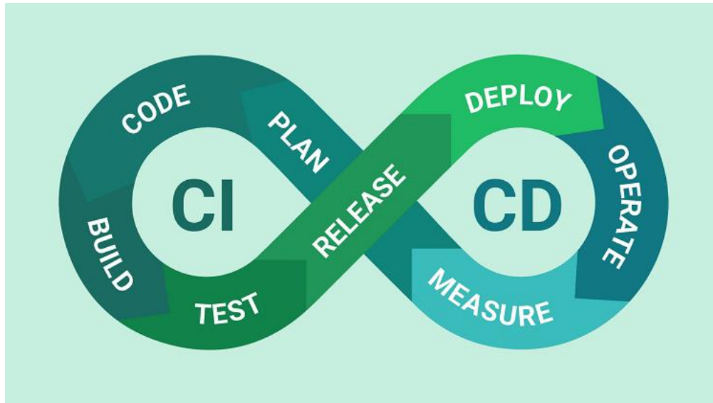
Figure 7 - 1 CI/CD
