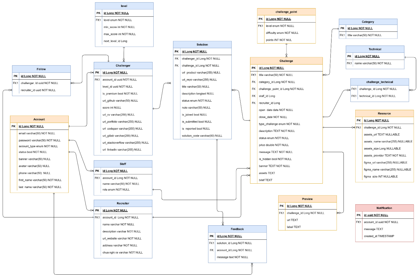
Figure 4 - 10 Class Diagram
